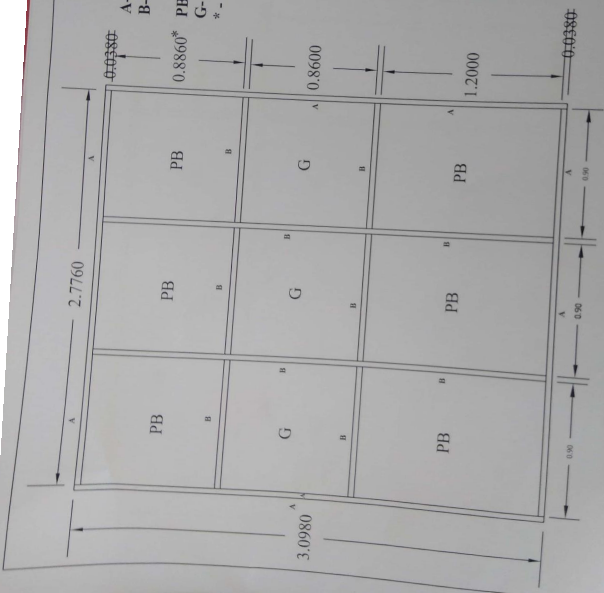
ALUMINIUM PARTITION (Internal Side)
