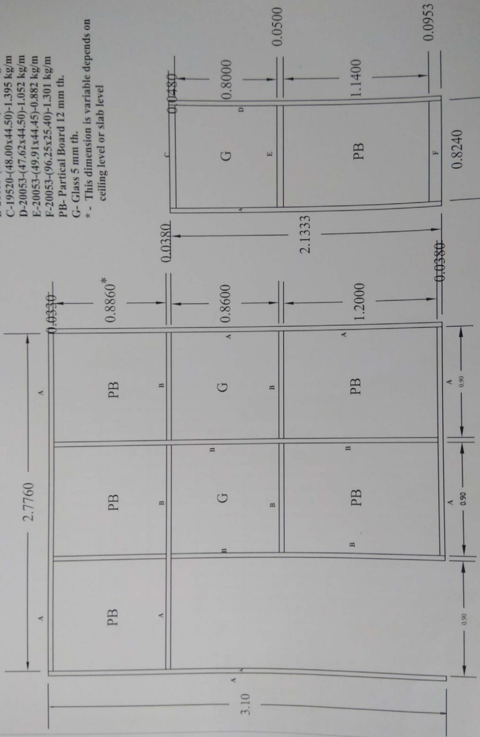
ALUMINIUM PARTITION (Door Side)
